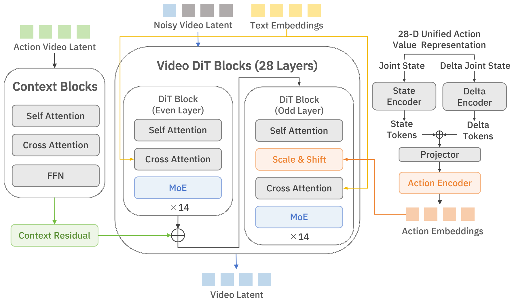
(a) Dual-Branch Action-Conditioned Video DiT
